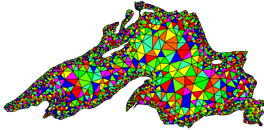
Random Partitioning
