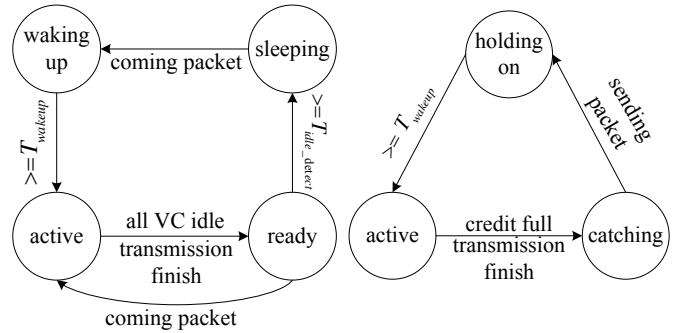
(a) Input controller states (b) Output controller states
