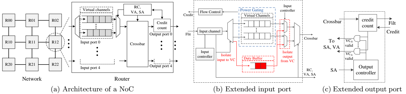
Figure 1: The NoC structure and extended input port and output port.
