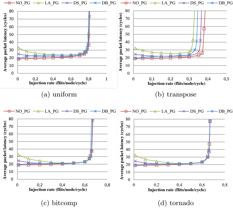
Figure 5: Packet latency across full range of workloads.
