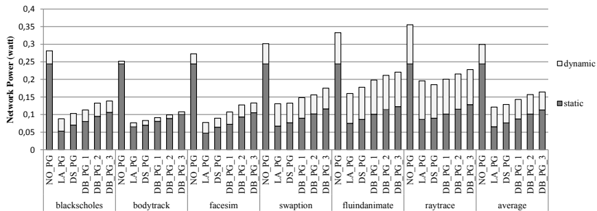
Figure 4: The breakdown of the NoC power consumption.
