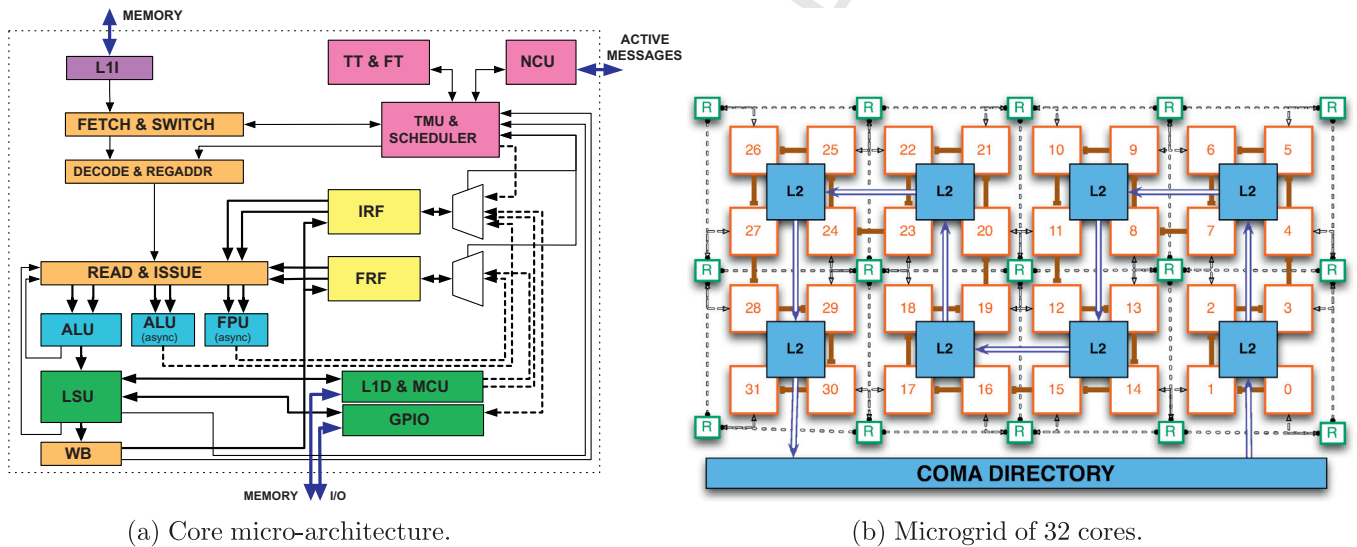
Fig. 2. Micro-architectural components.
