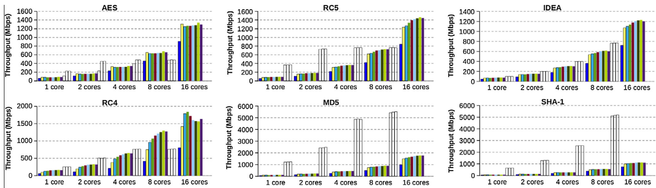
(a) Combined throughput for 1-8,16 streams per core on 1-16 cores (1-256 streams total). IXP2800 performance in leftmost 3 bars at each core group.
