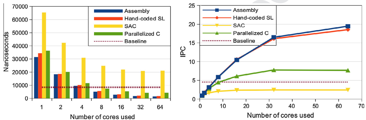
Fig. 7. Performance of the equation of state fragment.
