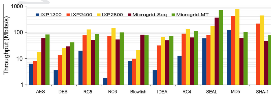
Fig. 8. Throughput for one stream on one core.
