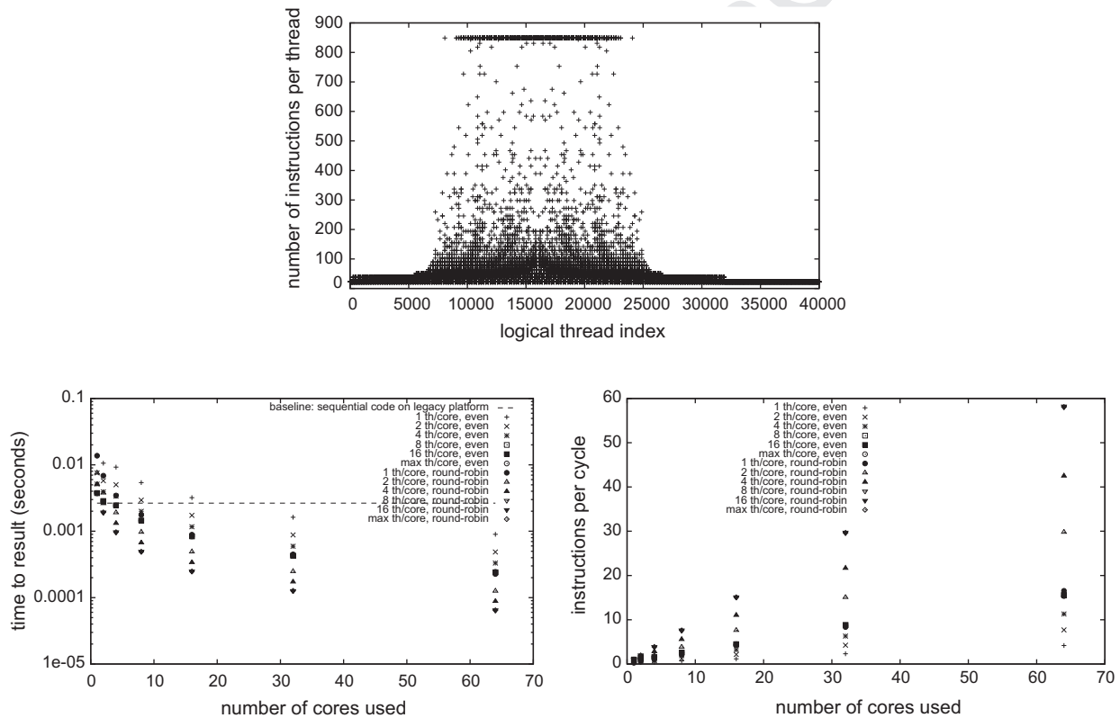
Fig. 5. Example heterogeneous workload: mandelbrot set approximation.
