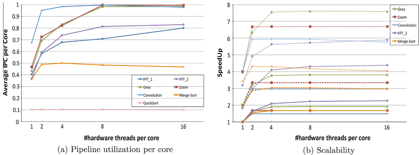
Fig. 4. Orthogonal benefits of multithreaded and multi-core execution.
