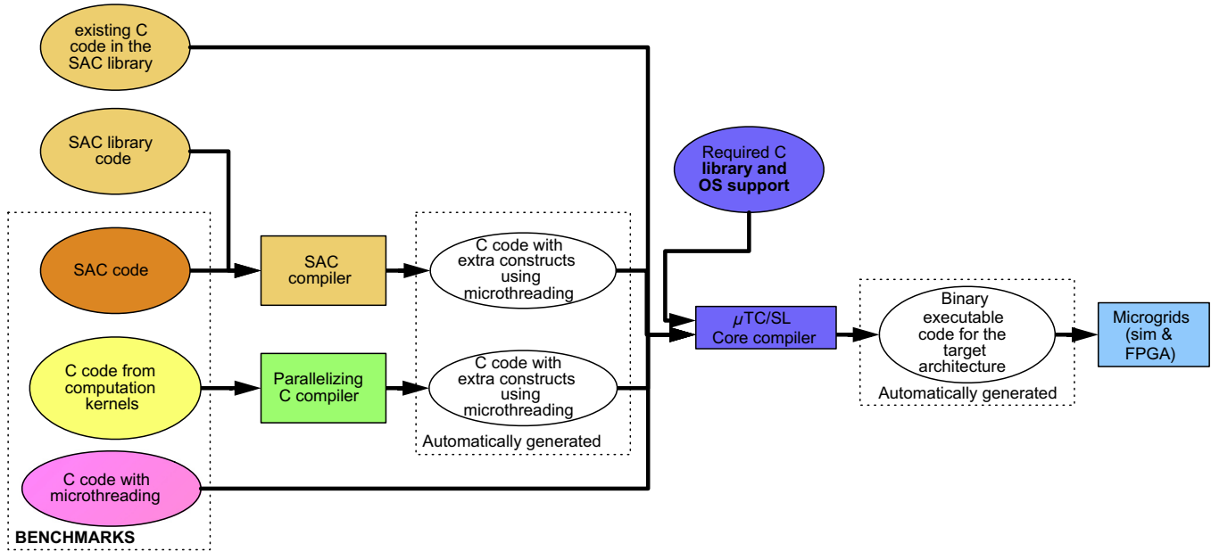
Fig. 1. The Apple-CORE software deliverables.
