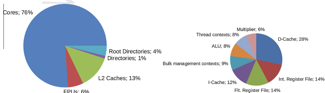
Fig. 3. Chip area breakdown: entire grid (left), per core (right).
