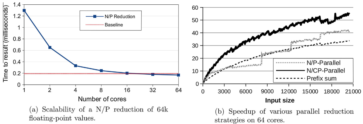
Fig. 6. Performance of parallel reductions.
