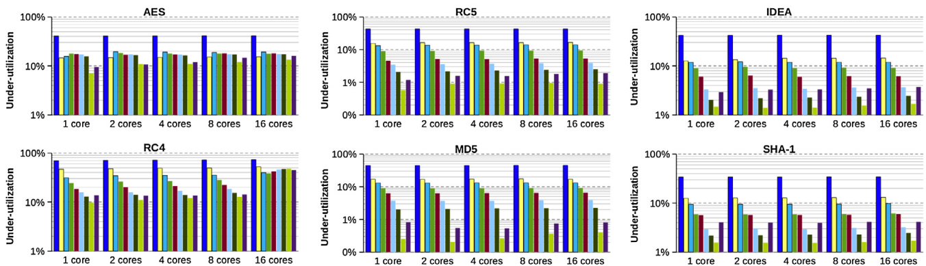
(b) Pipeline under-utilization.
