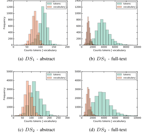
Fig. 2. Histograms of token and vocabulary frequencies for DS_1 and DS_2 for both abstract and full-text data. (b) and (d) contain very long tails for the number of tokens (up to 18,000).
