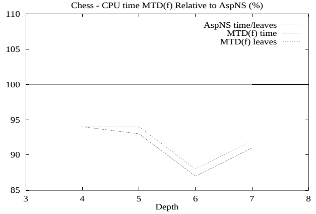
Figure 7: Execution time for Chess
