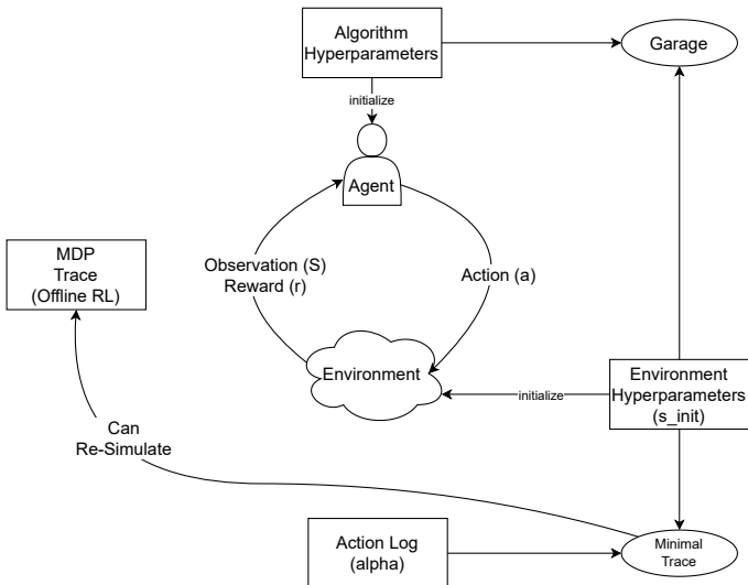
Fig. 1: A visualization of the relationship between reinforcement learning training, offline RL datasets (traces), minimal traces Garage [21], as well as the data collected for each.
