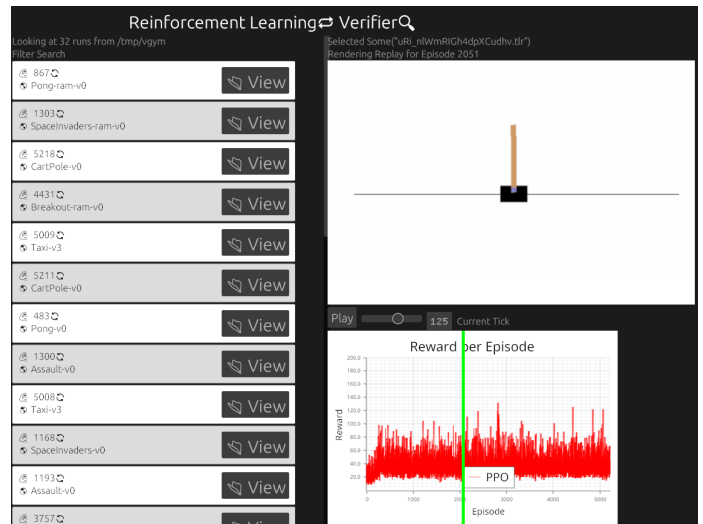
Fig. 3: Mock-up of a web-based tool we envision for future work. The left side contains a list of minimal traces, the environment, and amount of contained episodes. The right side shows details of the re-simulated trace. For inspection, one can select individual episode replays directly from the training reward graph, highlighted by the green vertical stripe. Each episode can be stepped through frame by frame.
