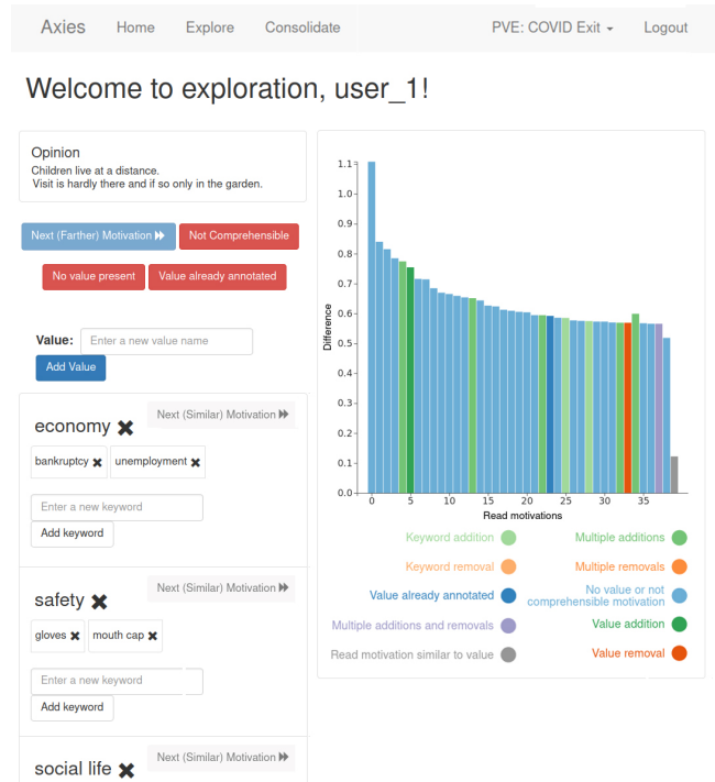
Figure 1: Exploration in the web application
