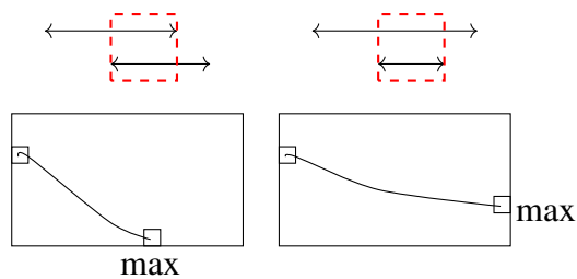
Figure 3: Semi-global alignment: finding overlap or containment.
