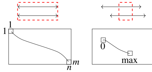
Figure 2: Global versus local alignment.
