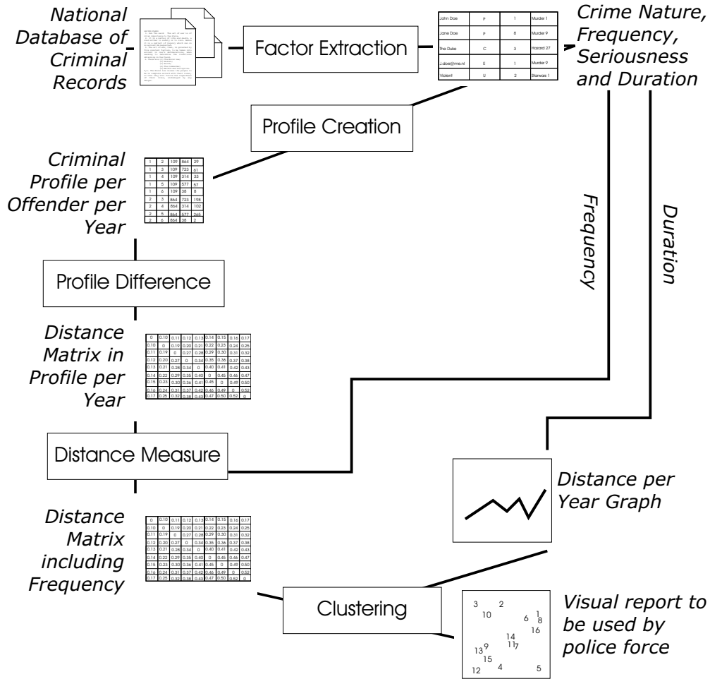
Fig. 1. Analysis of Criminal Careers
