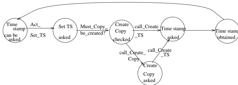
FIGURE 5.4.19. int-Set_TS: STD of the internal behaviour.
