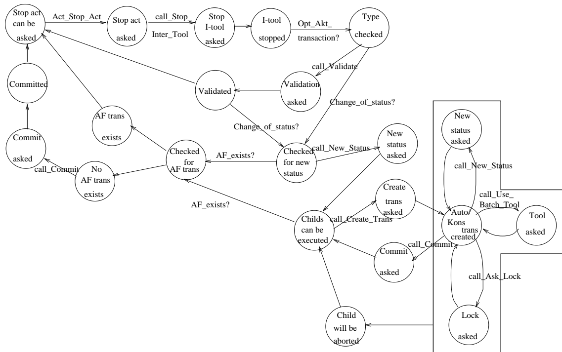
FIGURE 5.4.26. int-Stop_Act: STD of the internal behaviour.
