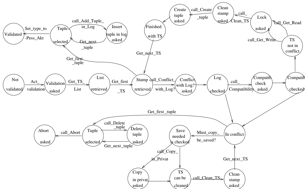
FIGURE 5.4.20. int-Validate: STD of the internal behaviour.
