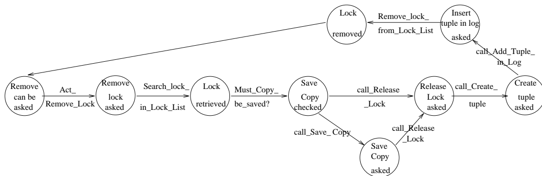
FIGURE 5.4.21. int-Remove_Lock: STD of the internal behaviour.
