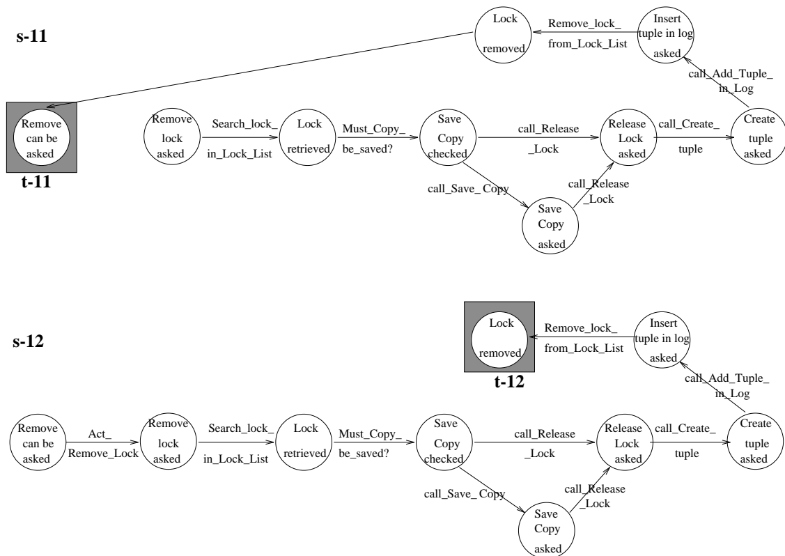
FIGURE 5.5.16. int-Remove_Lock's subprocesses and traps w.r.t. Pass_AF Transaction.
