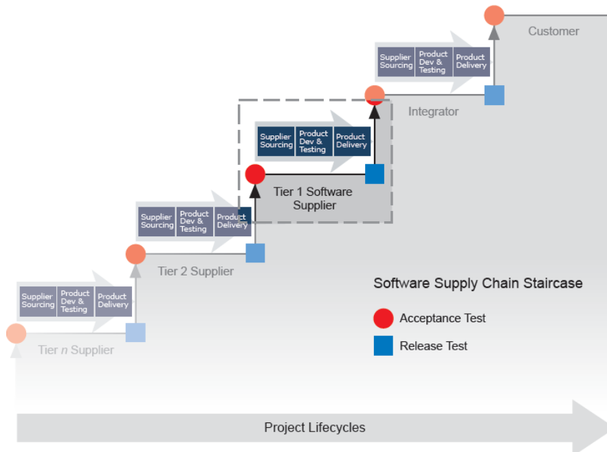
Figure 11: The Software Supply Chain resembles a staircase, where each step holds a different supplier. (SAFECD)E
