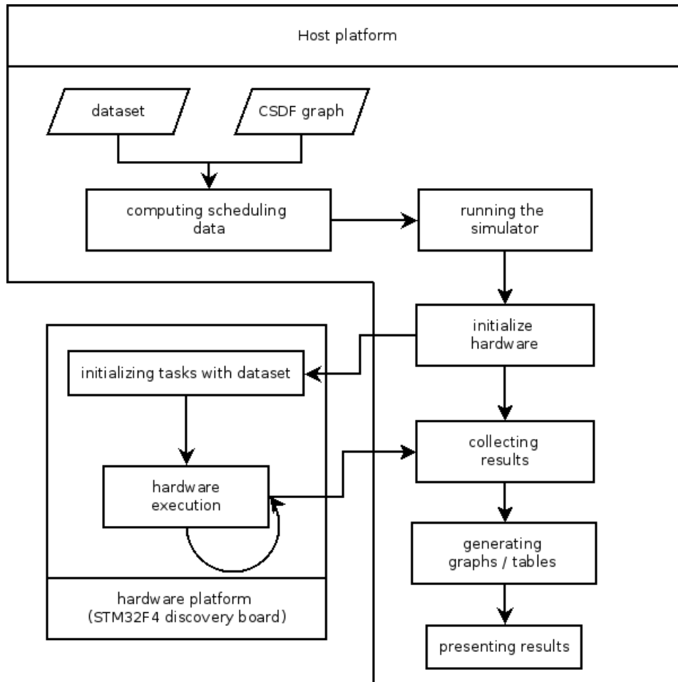
Figure 3.1: Schematic overview of the framework, each box represent a separate stage within the framework.
