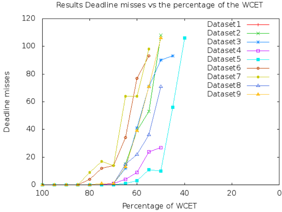
Figure 4.1: Deadline misses versus percentage of the WCET for all datasets
