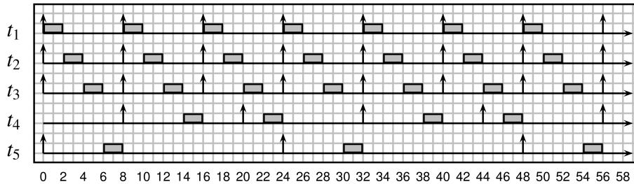
Figure 2.3: Example of a schedule.
