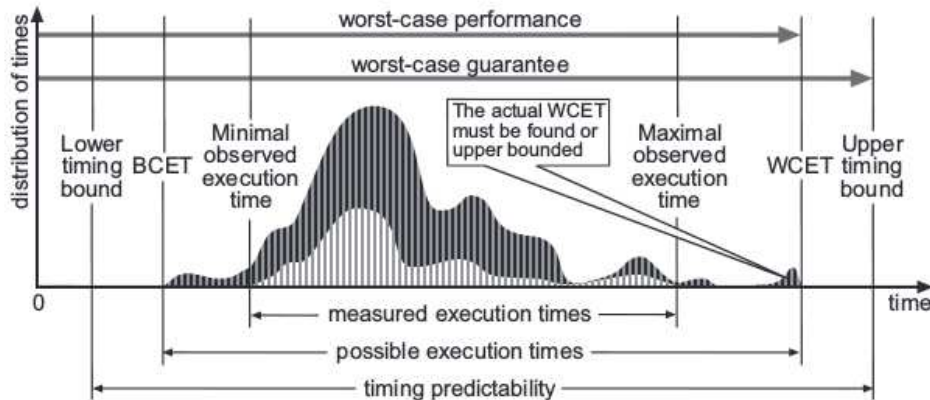
Figure 2.1: Timing analysis of systems.(Figure by Reinhard Wilhelm et al. [WEE + 08]).
