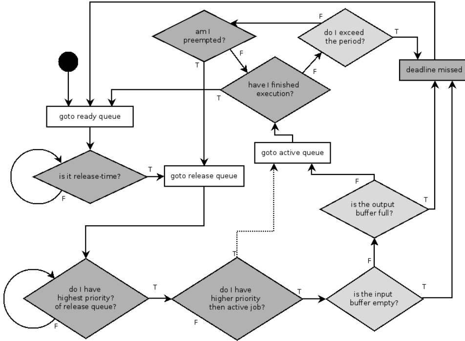
Figure 3.4: Lifecycle of a task within a system
