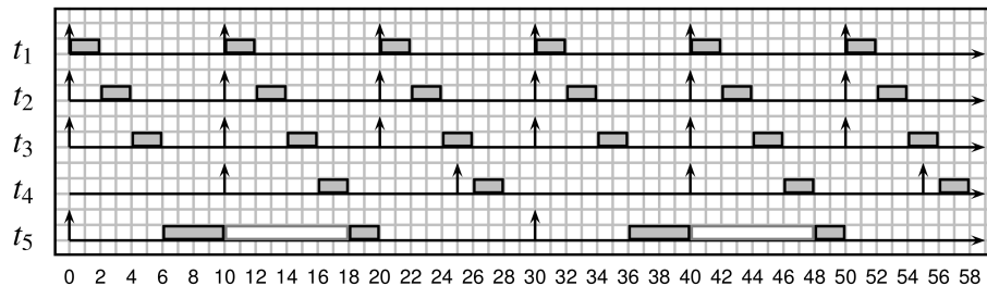
Figure 2.4: Example of a schedule with preemption.
