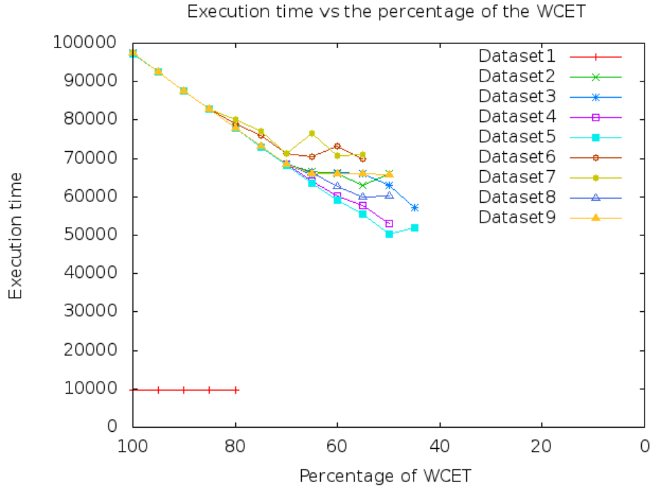
Figure 4.2: Troughput versus percentage of the WCET for all datasets
