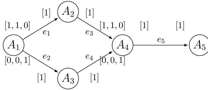
Figure 3.2: CSDF graph containing 5 actors and 5 edges.
