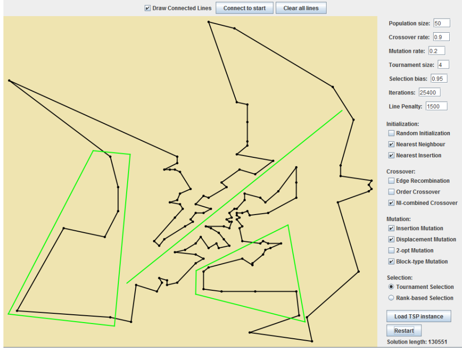
Figure 5: A solution of the solver on the bier127 problem with area constraints.
