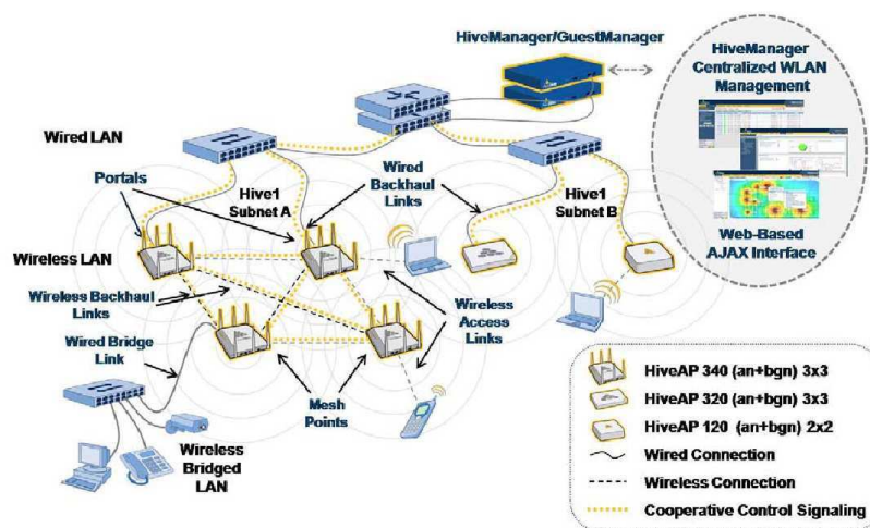
Figure 10: Overview of the Aerohive components[1]
